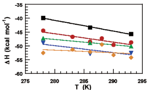
Figure 2. Plot of \Delta H versus temperature used to determine \Delta C_p for duplex 1 formation in 50 mM HEPES, pH 7.5 as a function of added NaCl: 100 mM (orange \blacklozenge ), 300 mM (green \blacktriangle ), 500 mM (blue \blacktriangledown ), 1 M (red \bullet ), 1.5 M (black \blacksquare ). Data points are the mean of three independent trials.
