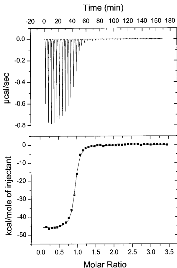
Figure 1. Typical data from an ITC experiment. A 75 \mu\text{M} solution of strand 1B was titrated into 1.4 \text{ mL} of 5 \mu\text{M} strand 1A equilibrated at 15 °C. Both RNAs were in 50 \text{ mM} HEPES, pH 7.5 and 1 \text{ M} NaCl. This run yielded fitting parameters: \Delta H = -46.1 \pm 0.2 \text{ kcal mol}^{-1} ; \Delta S = -125 \text{ cal mol}^{-1} \text{ K}^{-1} ; K_a = 4.3 \times 10^7 \text{ M}^{-1} ; N = 0.91 \pm 0.01 .
